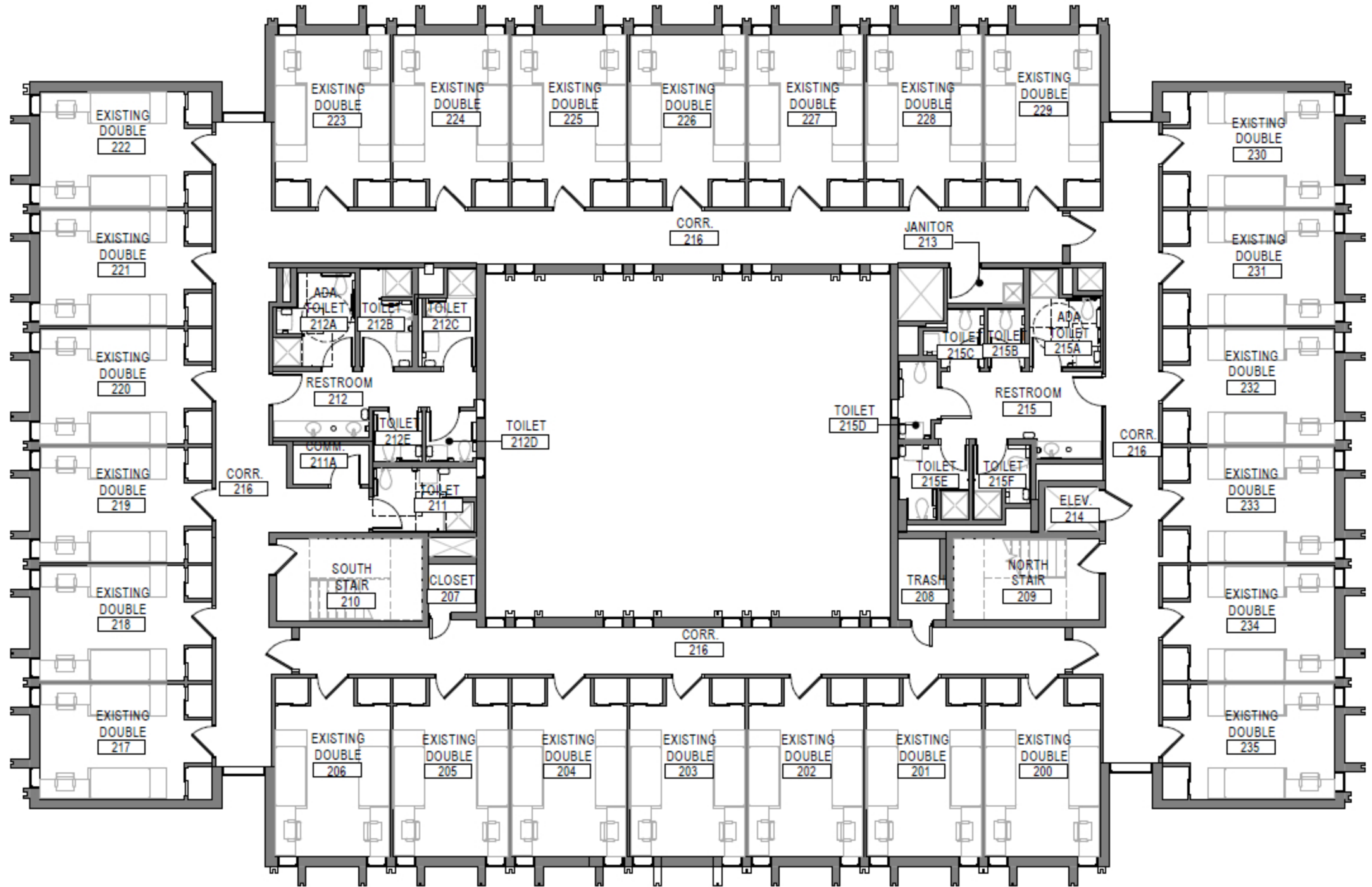
2 BARNHARDT FLOOR PLAN - LEVEL 02 & 03 - NEW 3 3/32" = 1'-0"
